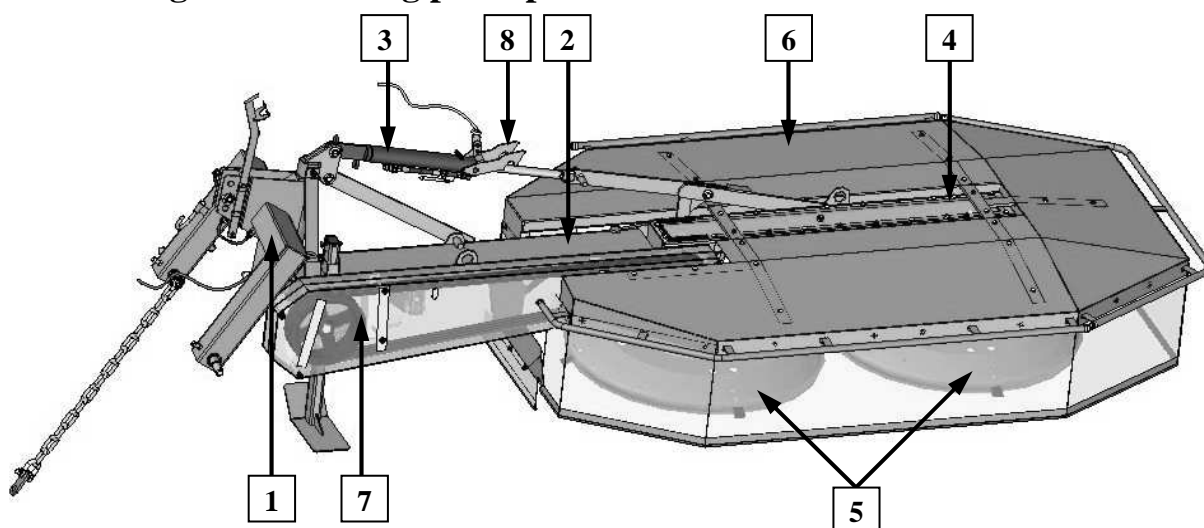
Fig. 2. Parts of SaMASZ rear drum mower – flat cover
