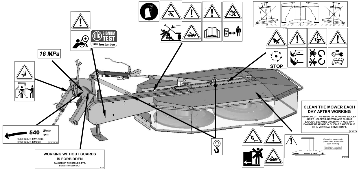
Fig. 7a. Warning decals placed on the mower (Z 010, Z 010/1, Z 010/2)
