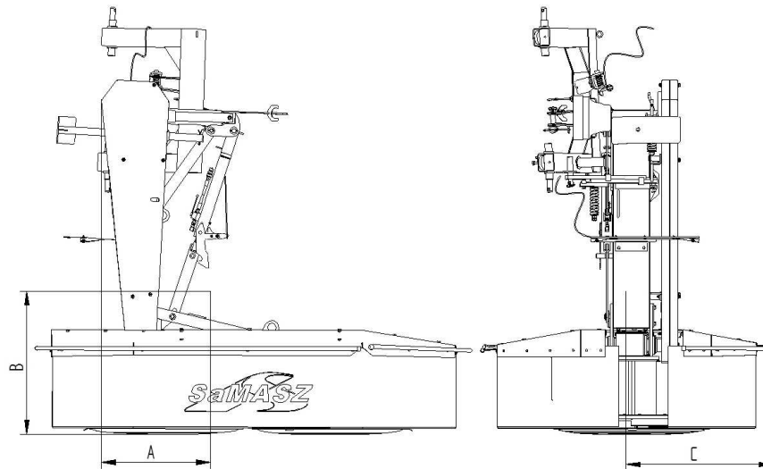
Fig. 5. Transport holders
