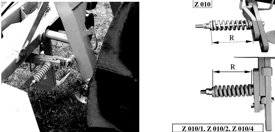
Fig. 8. Safety breakaway device
