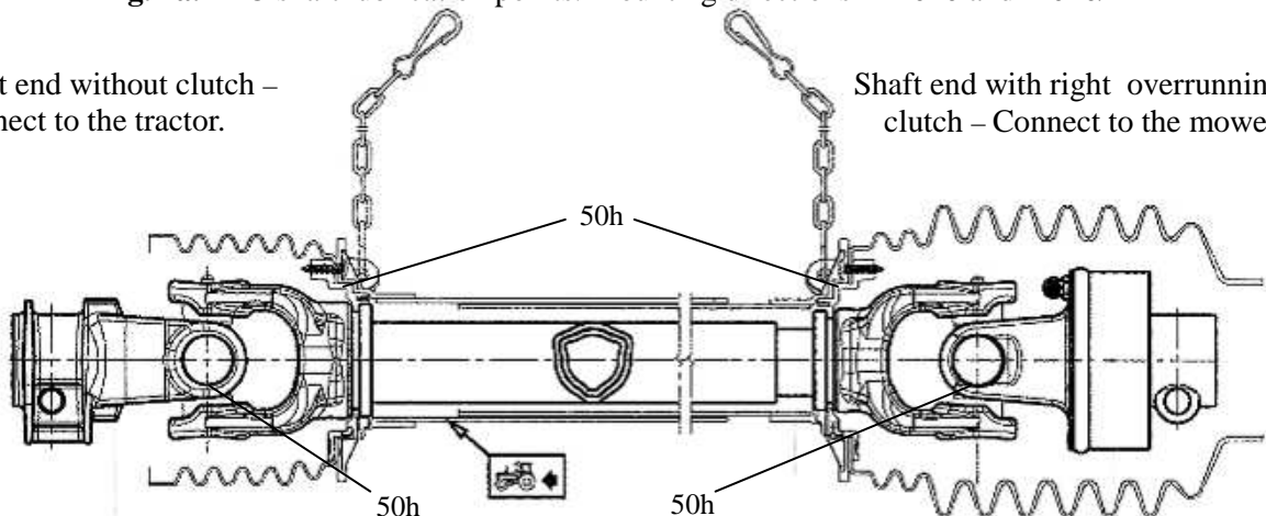
Fig. 4b. PTO shaft lubrication points. Mounting directions – Z 010/2 and Z 010/4
