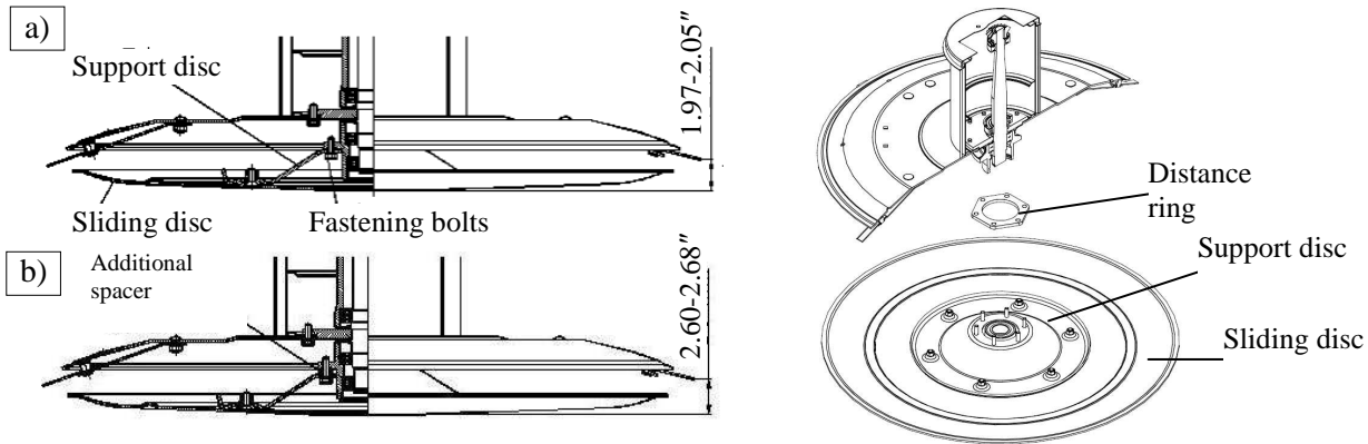
Fig. 27. Adjusting the cutting height by fitting or removing the distance ring
