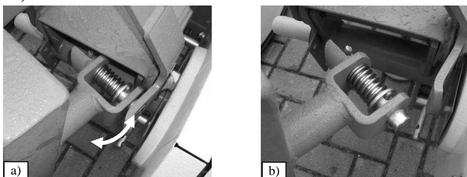
Fig. 10. Mower's transport lock a) transport position, b) working position
