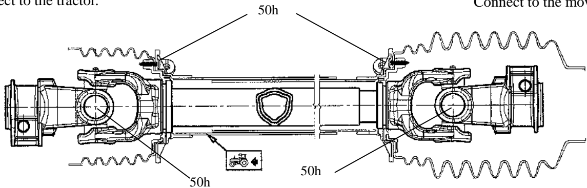
Fig. 4a. PTO shaft lubrication points. Mounting directions – Z 010 and Z 010/1
